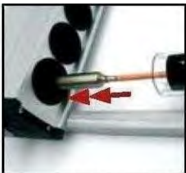
17. Push the heat pipe condenser to the manifold hole, make sure the condenser touch the heat pipe manifold port tightly
