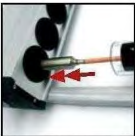
13. Push the heat pipe condenser to the manifold hole, make sure the condenser touch the heat pipe manifold port tightly
