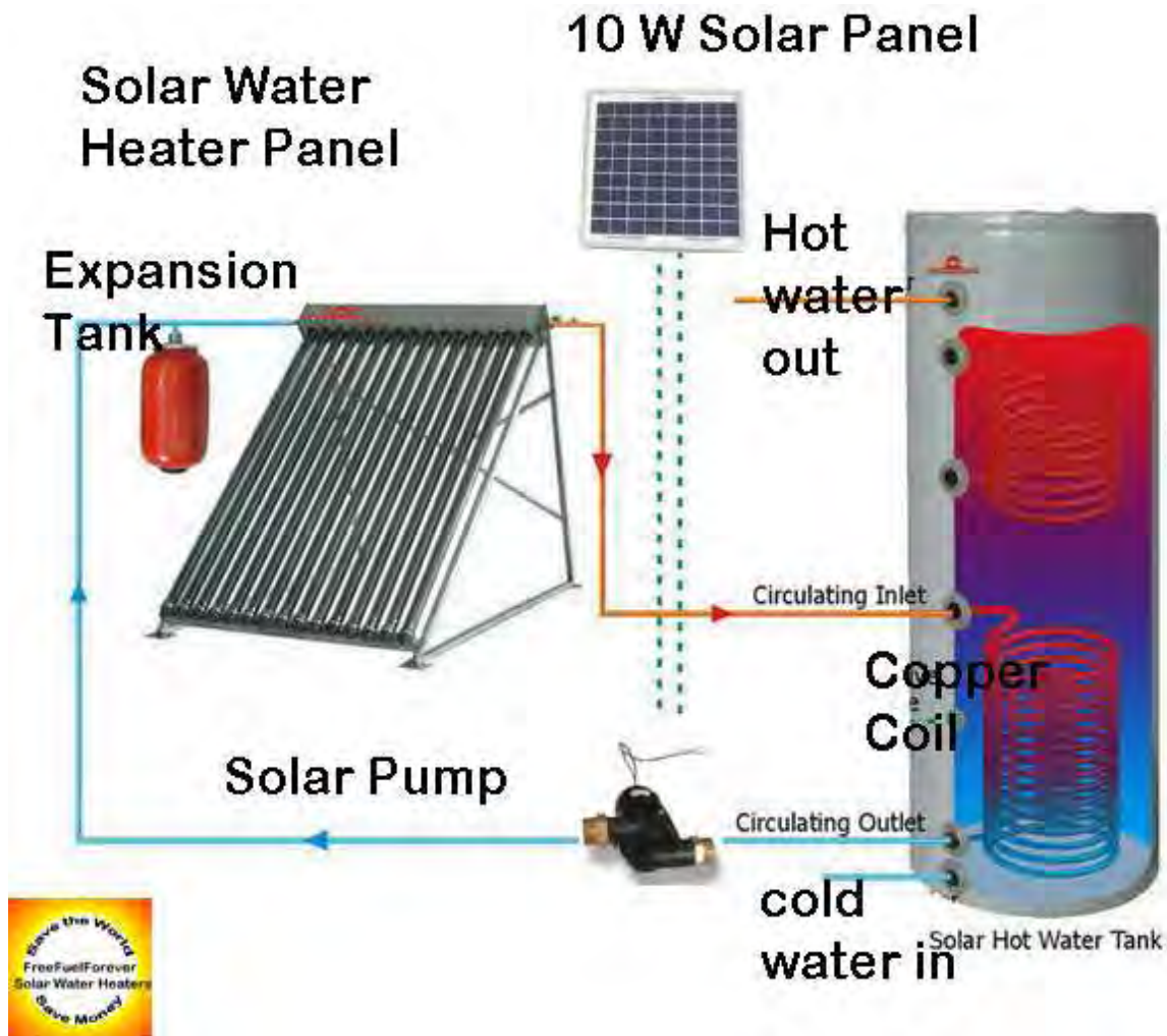
Illustration 3: Photovoltaic direct circulation pump driving a simple split solar water system
